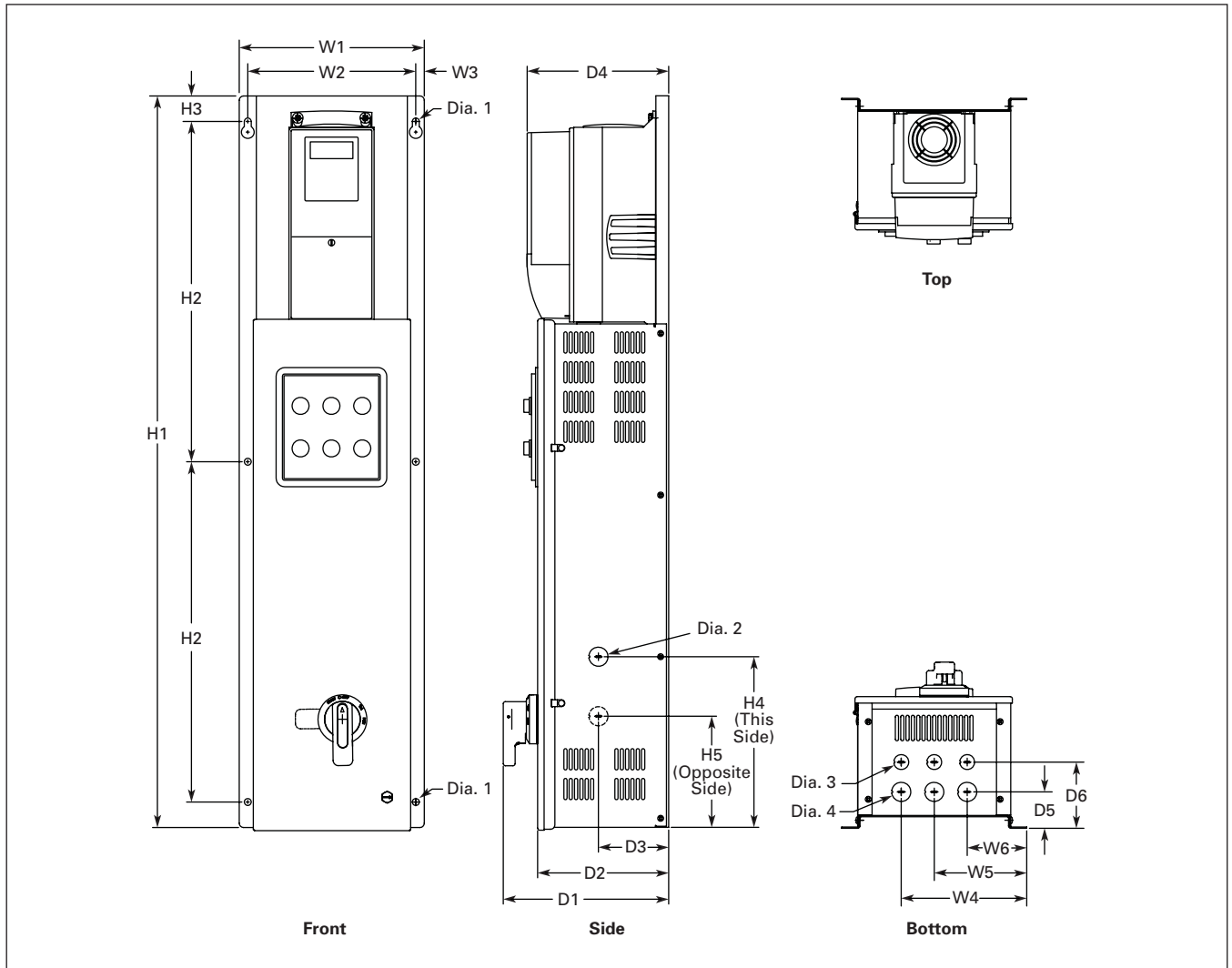
Figure 6. Approximate Dimensions
