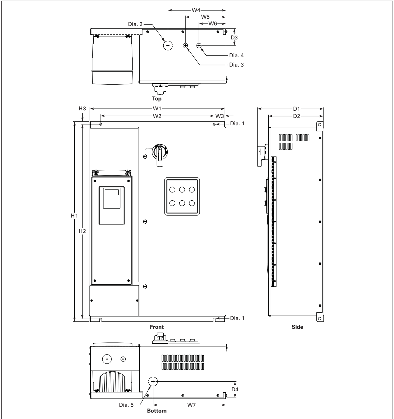
Figure 10. Approximate Dimensions
